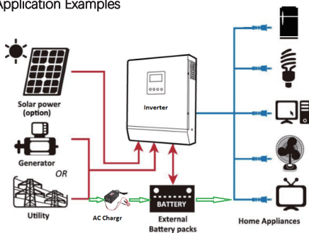
Hybrid Power System Figure
